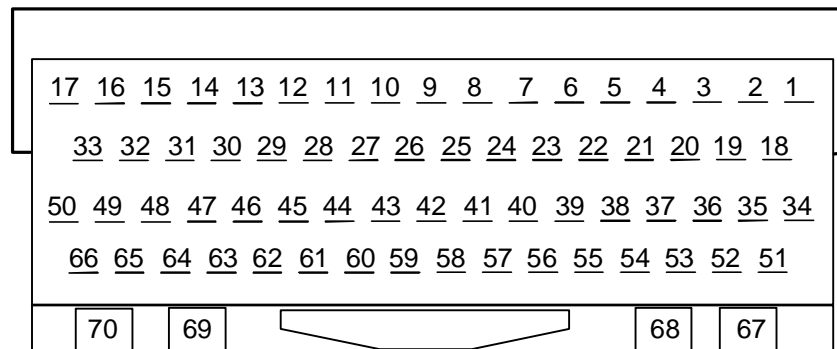
“E” CONNECTOR FACE VIEW
