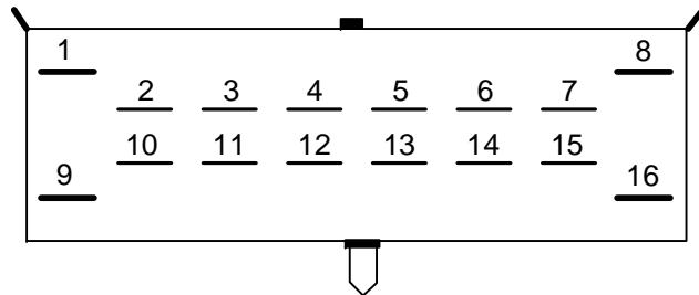
“VPWR” CONNECTOR FACE VIEW
